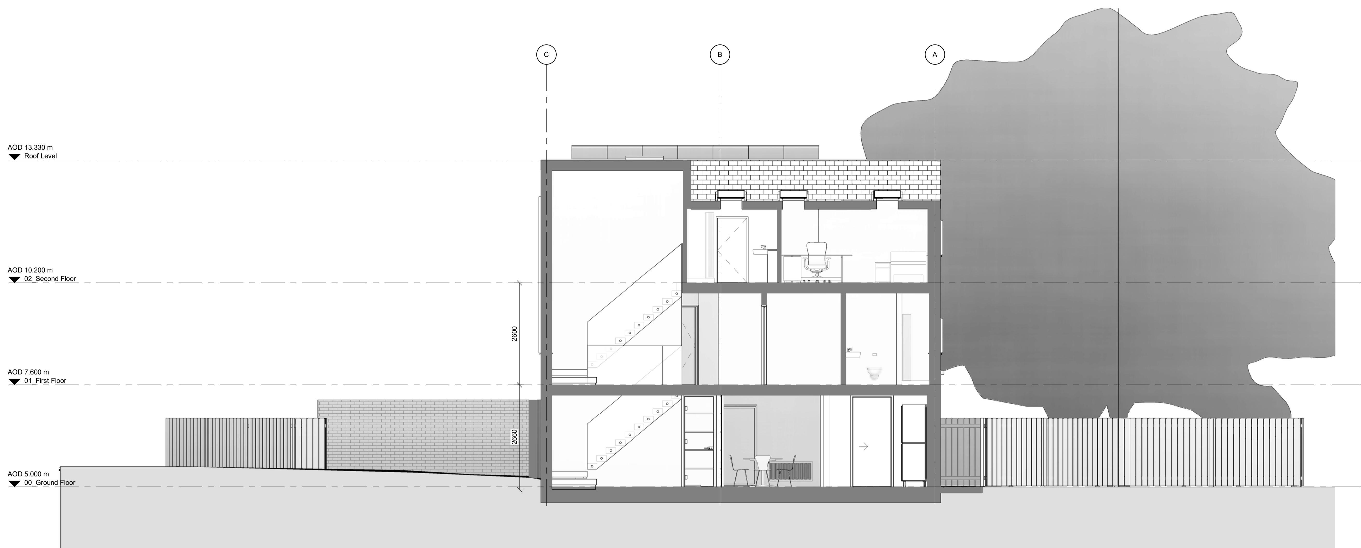
1 Proposed Section C-C 20352 1 : 50
