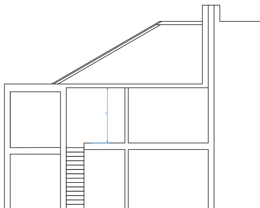
SECTION CC AS EXISTING
