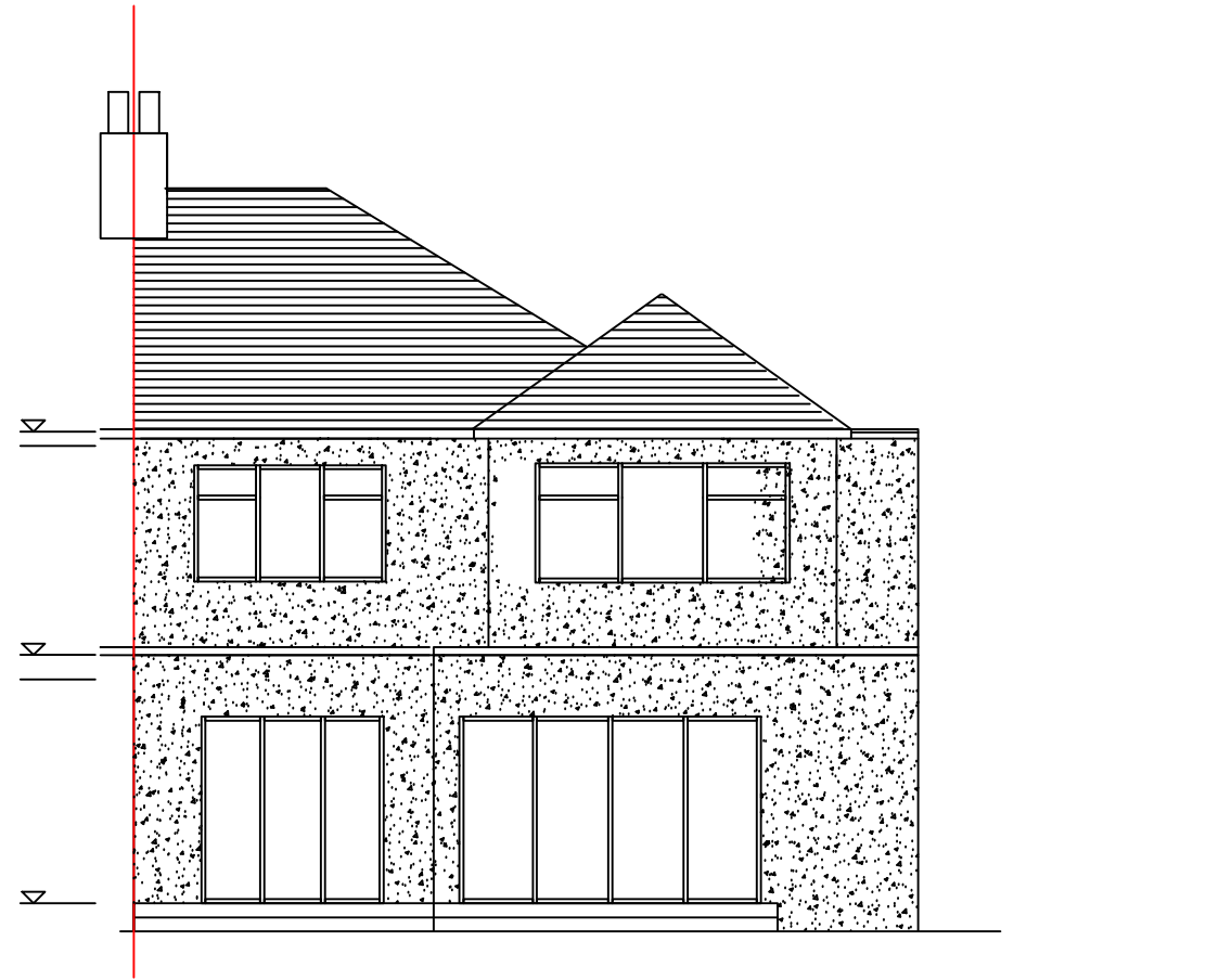
REAR ELEVATION AS EXISTING
