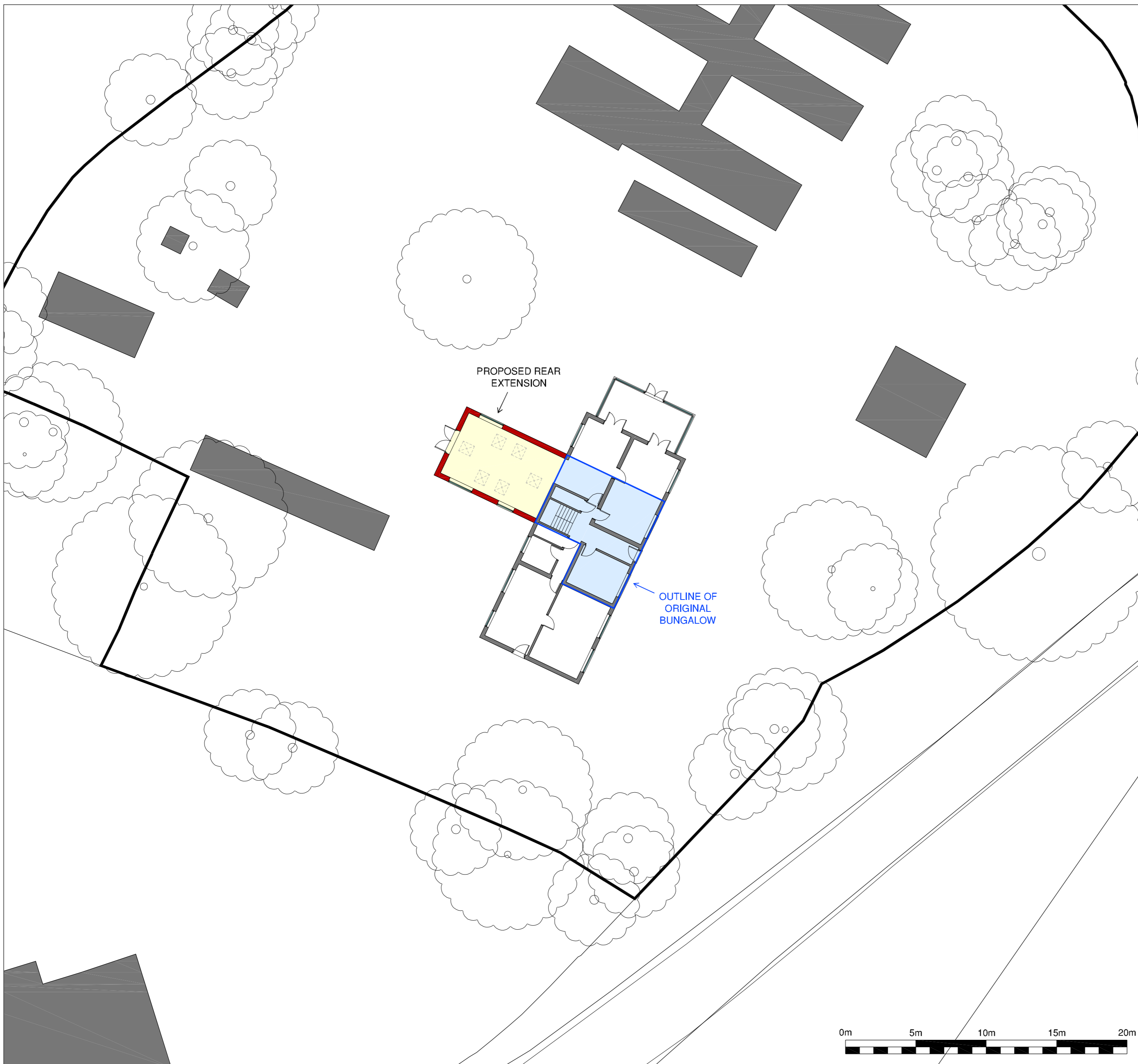
PROPOSED SITE LAYOUT (1:200)
