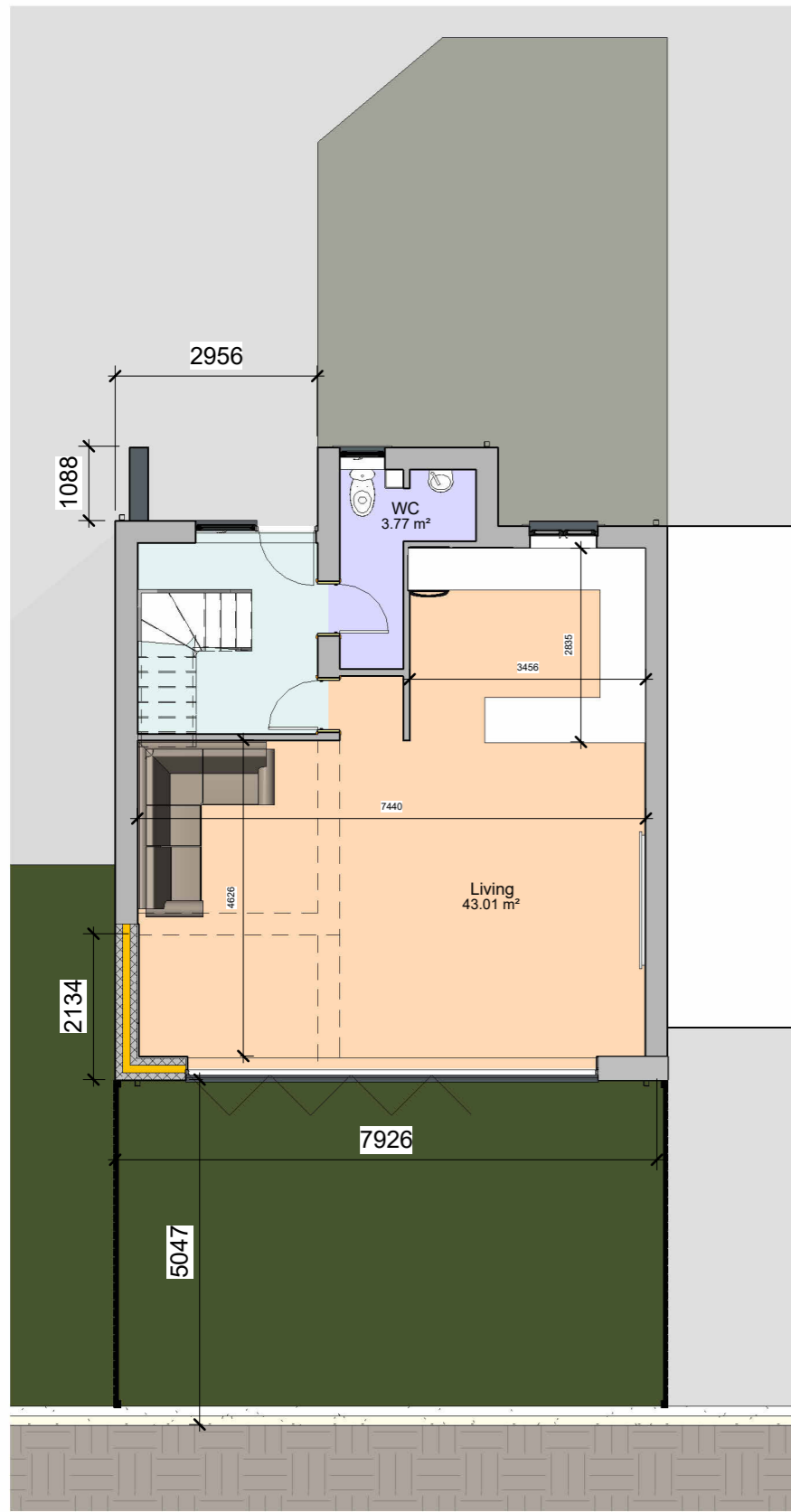
1 Ground Floor 1 : 100
