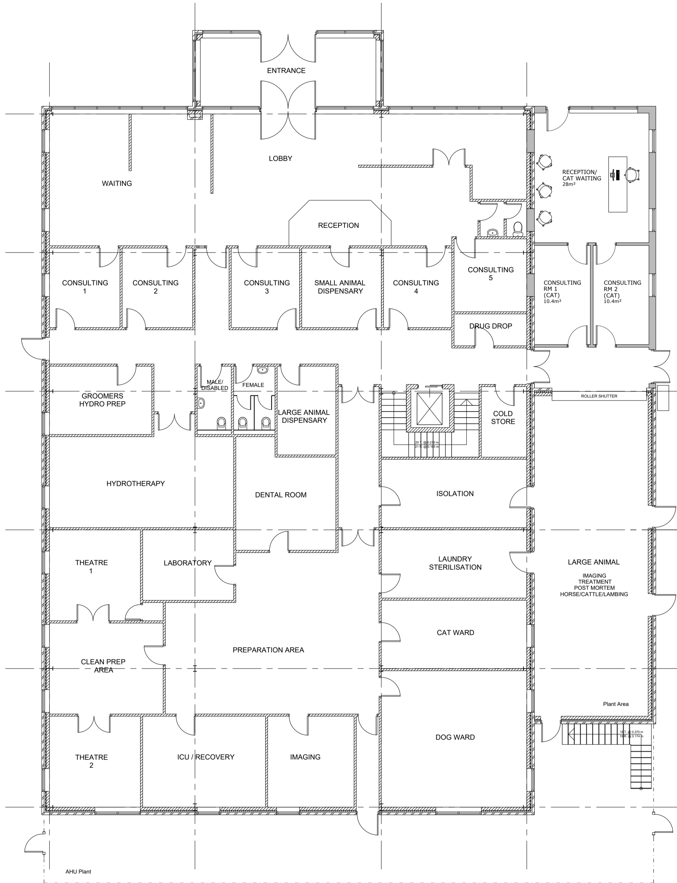
01 PROPOSED GROUND FLOOR PLAN 1:100
