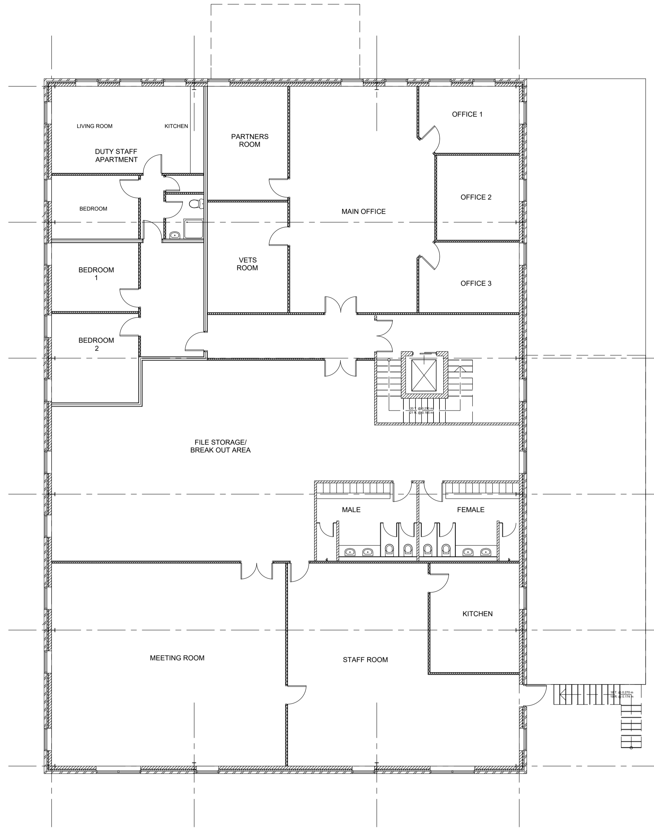
02 PROPOSED FIRST FLOOR PLAN 1:100
