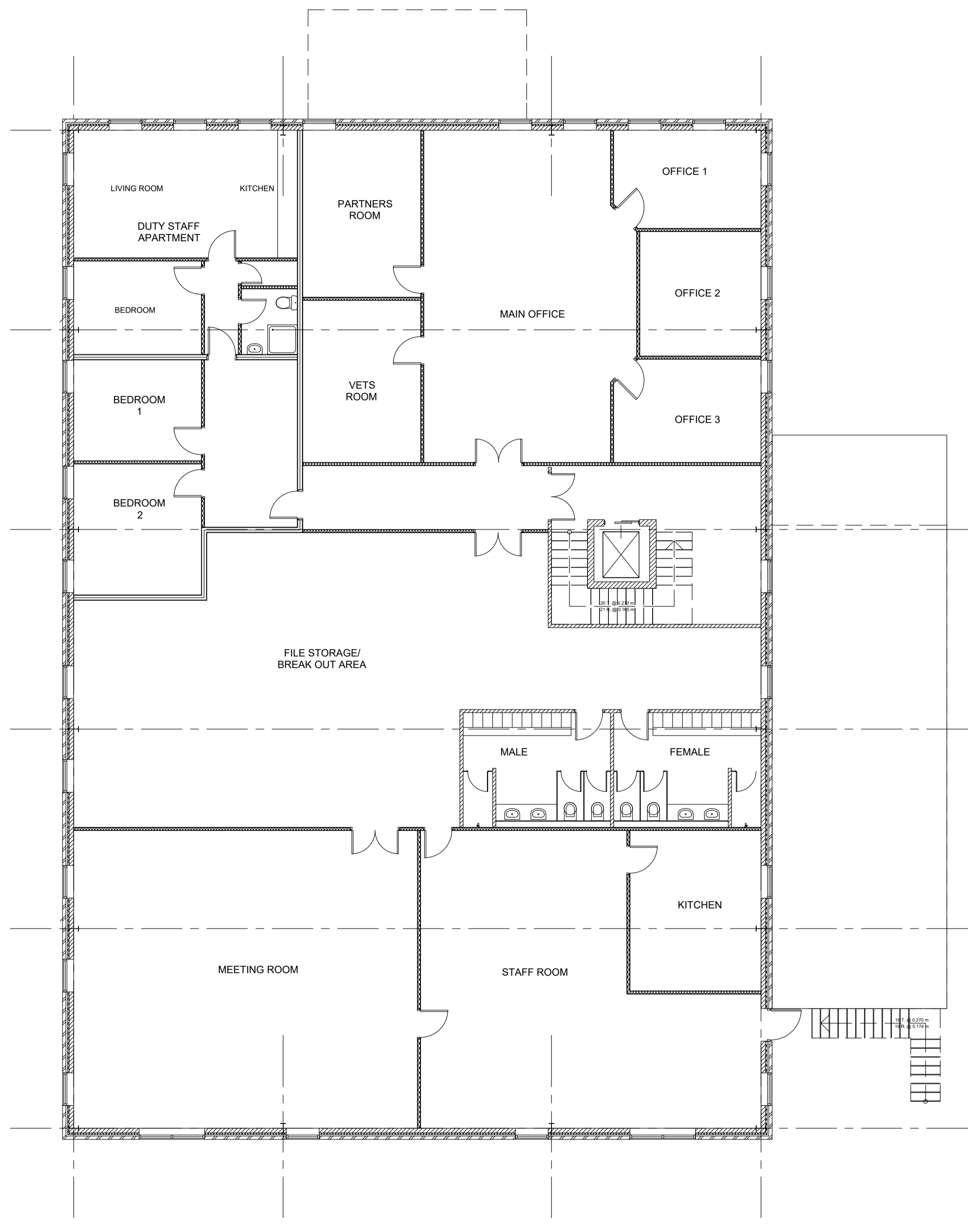
02 EXISTING FIRST FLOOR PLAN 1:100
