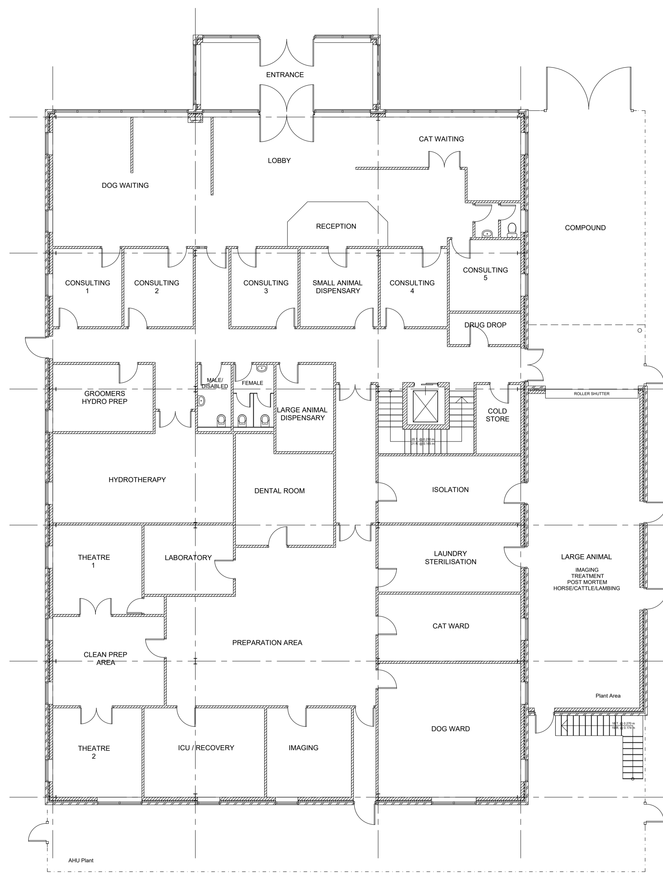
01 EXISTING GROUND FLOOR PLAN 1:100
