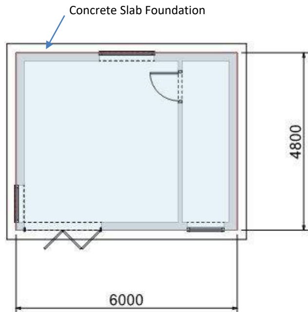
Proposed Floor Plan – 1:100
