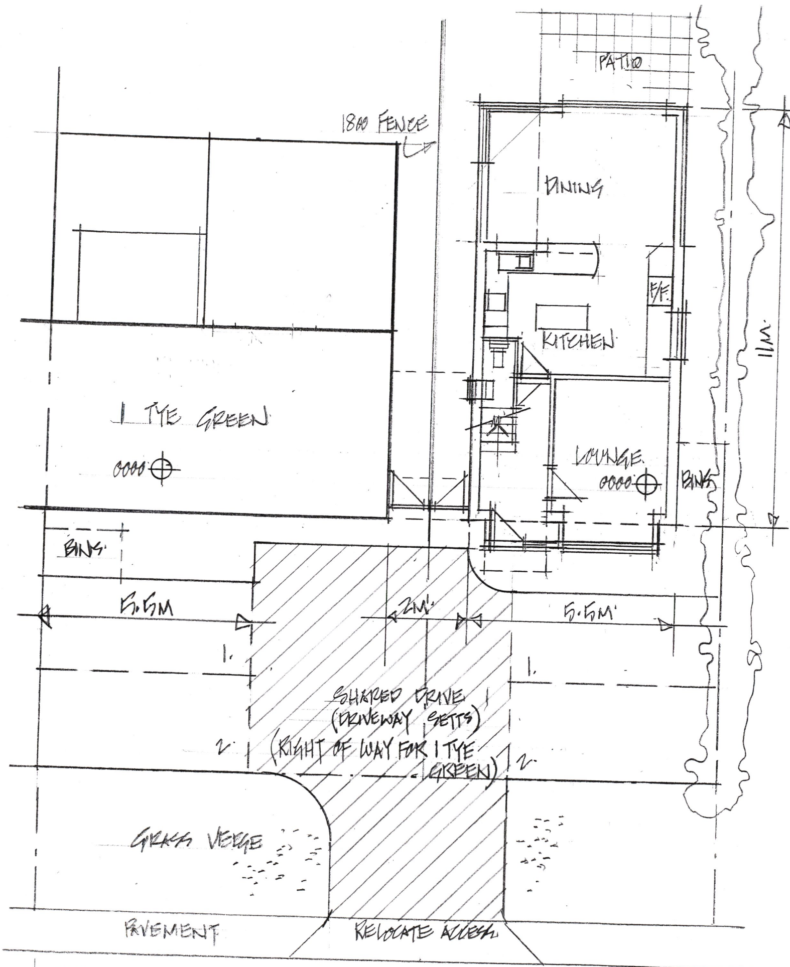
GROUND FLOOR (SITE LAYOUT) 1:100
