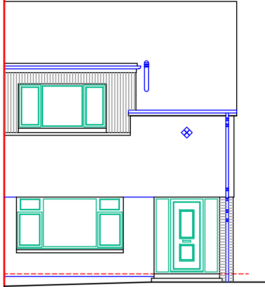
Front Elevation
