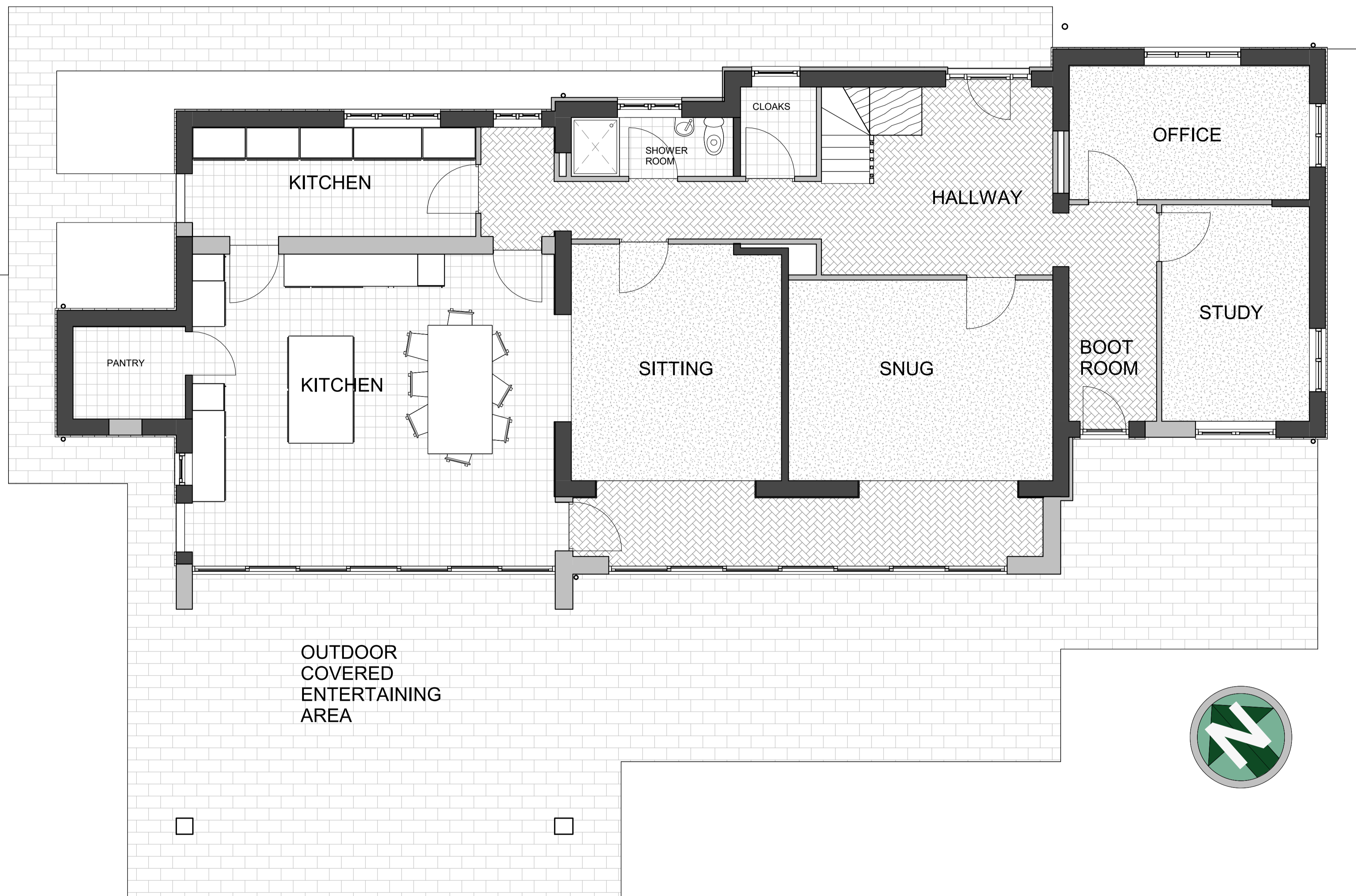
1 00 Ground Floor GA (RIBA Stage 3) 1 : 50
