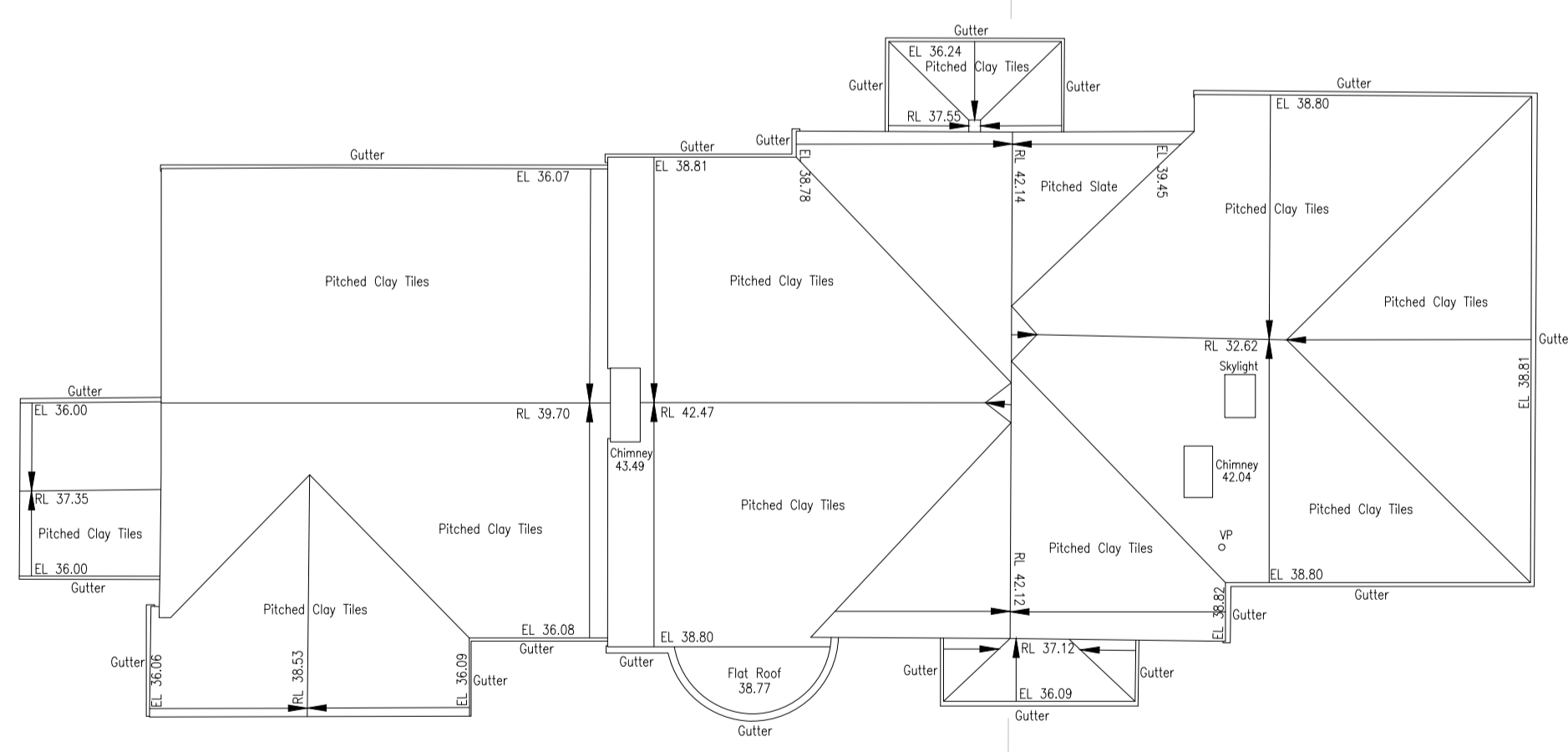
ROOF PLAN
