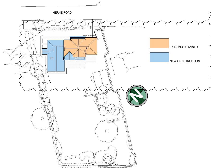
1 03 Roof Plan (RIBA Stage 3) 1 : 250
