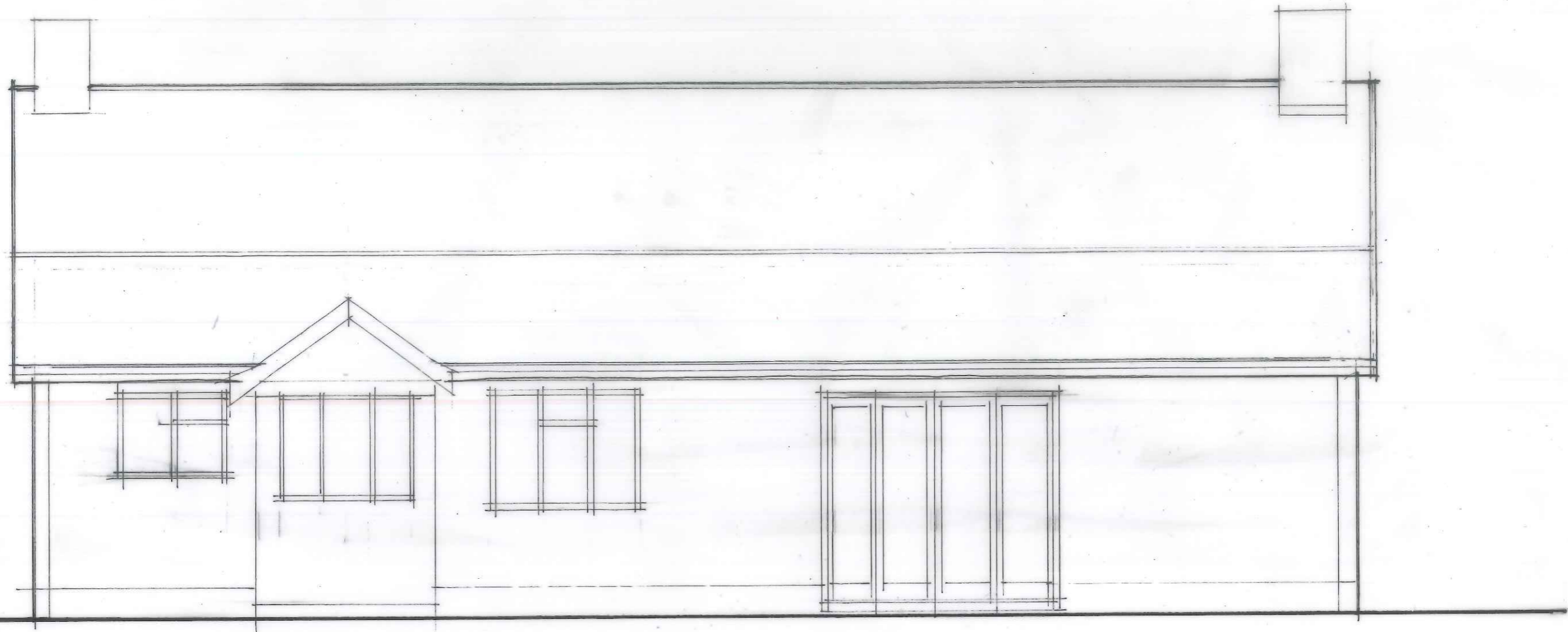
REAR ELEVATION
