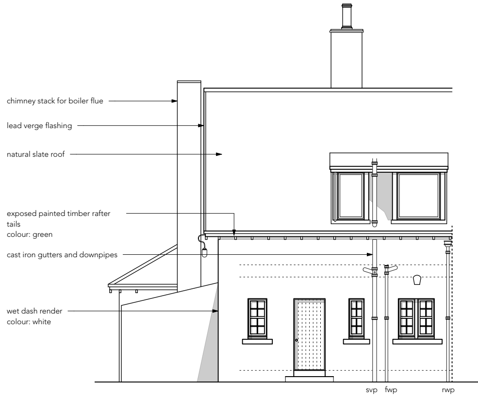
west elevation
