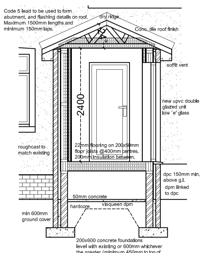
Section 1:50
