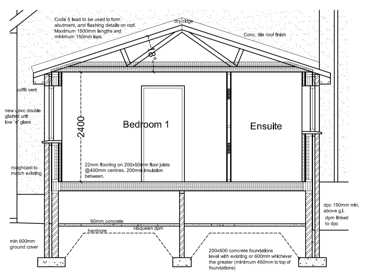
Section 1:50
