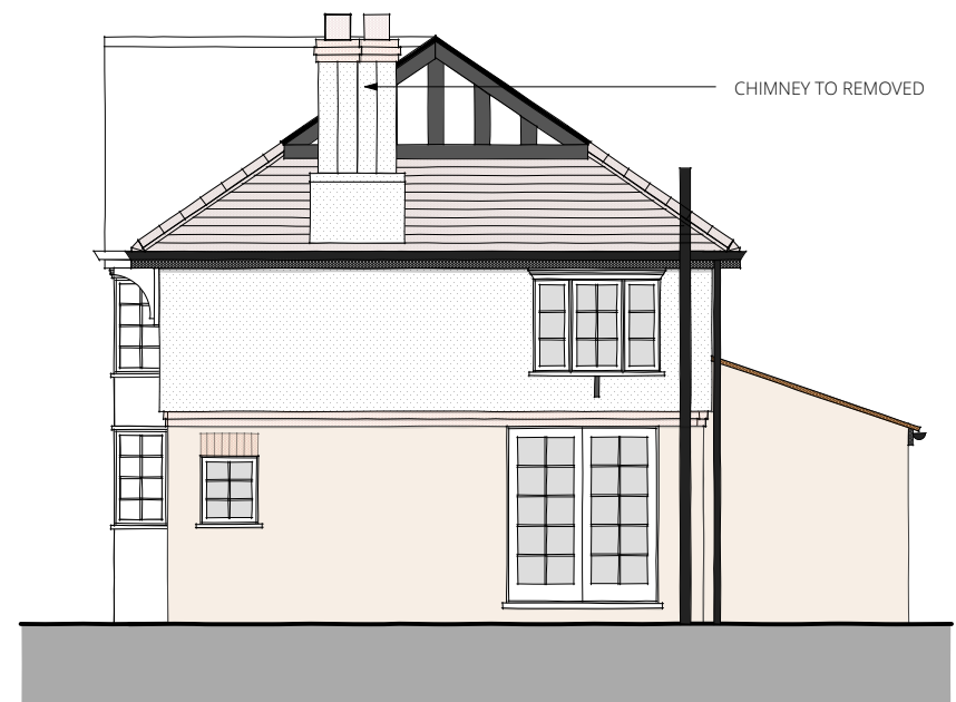
ELEVATION 03
