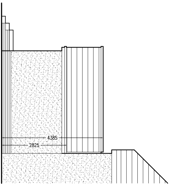
PROPOSED SIDE (NE) ELEVATION 1:100 @ A3
