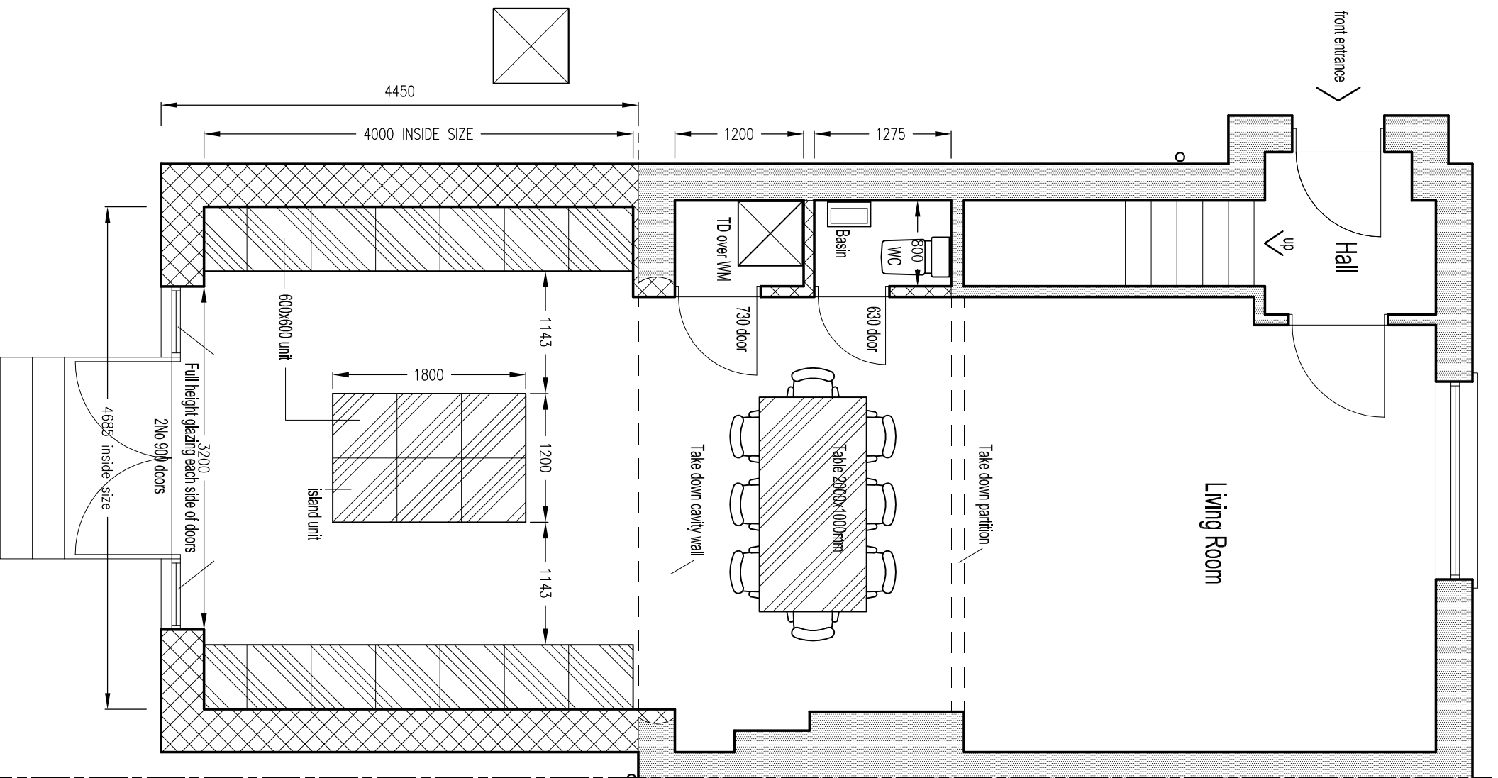
PROPOSED GROUND FLOOR PLAN 1:50 @ A3
