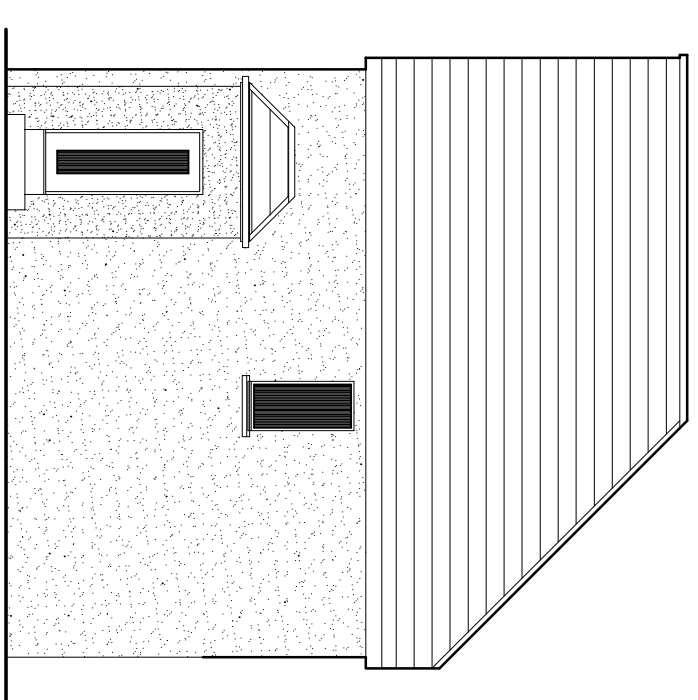
EXISTING SIDE (SW) ELEVATION 1 : 100 @ A3
