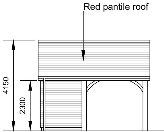
North (Front) Elevation
