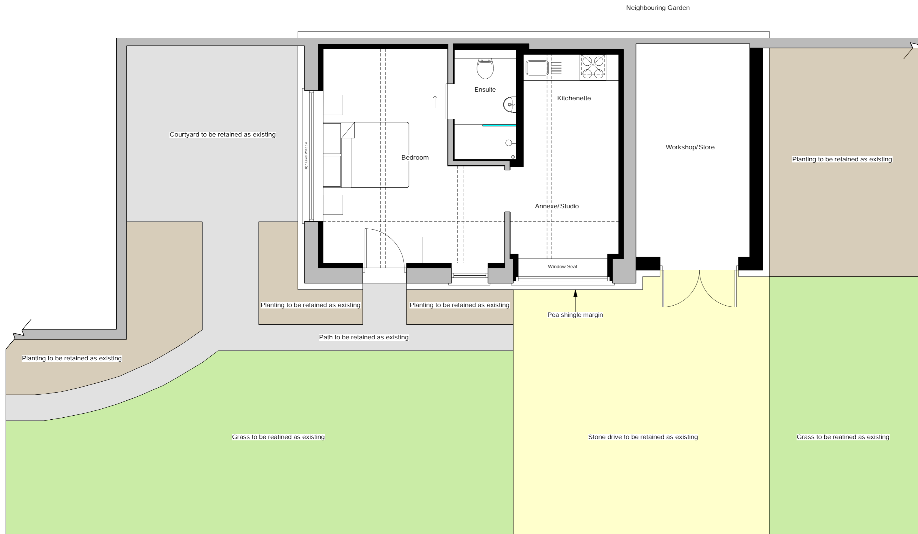
Proposed Landscape Plan Scale 1:50
