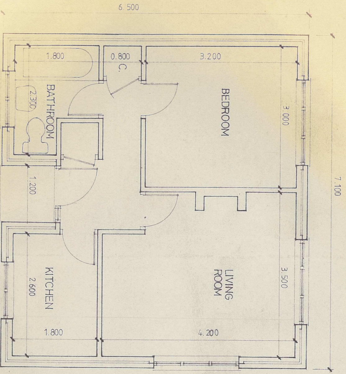
FLOOR PLAN 1:50
