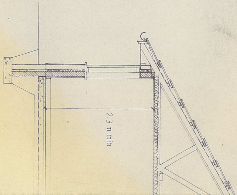
TYPICAL SECTION
