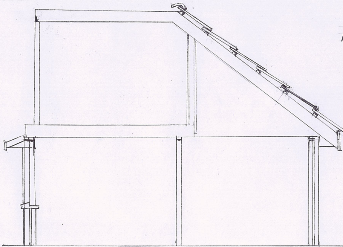
CROSS SECTION 1:50
