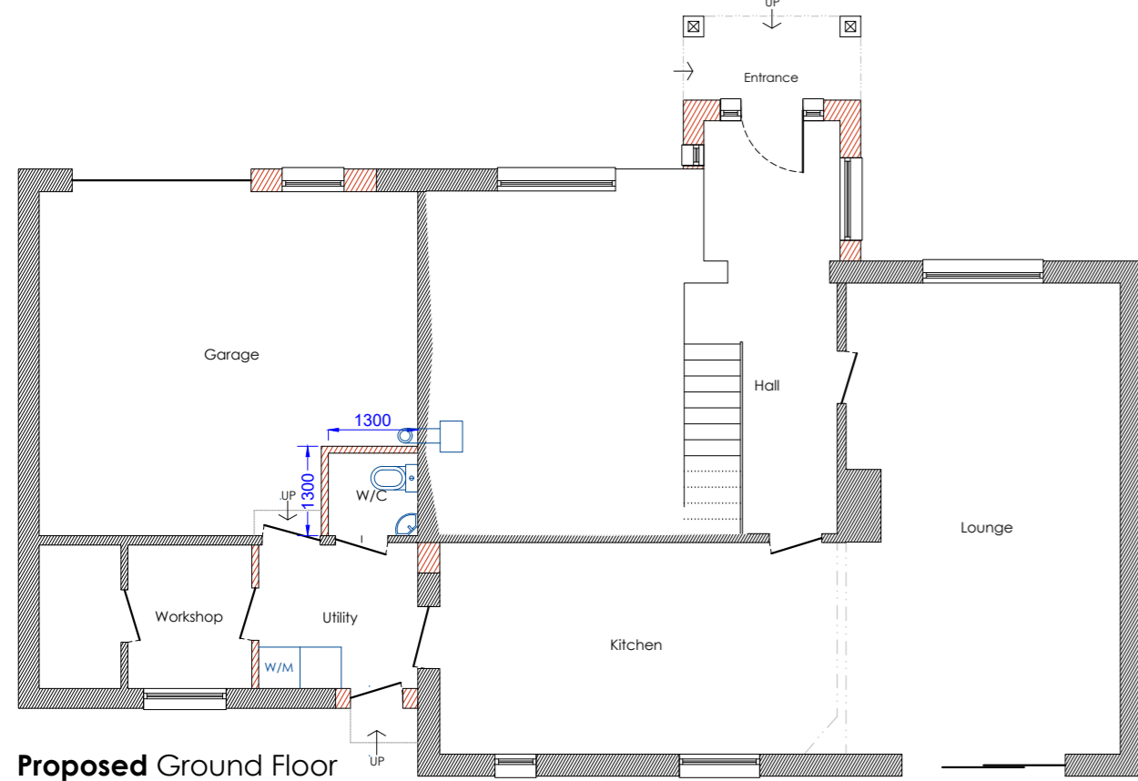
Proposed Ground Floor scale 1:100
