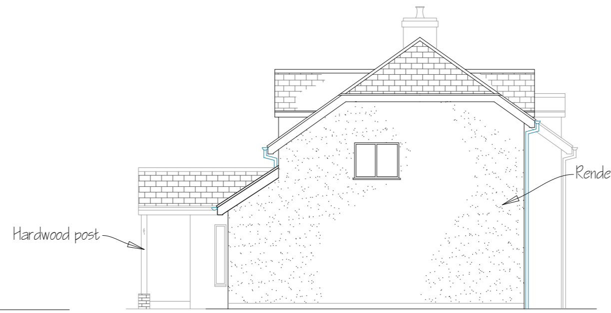
East scale 1:100
