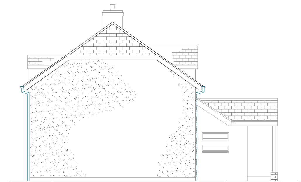
West scale 1:100
