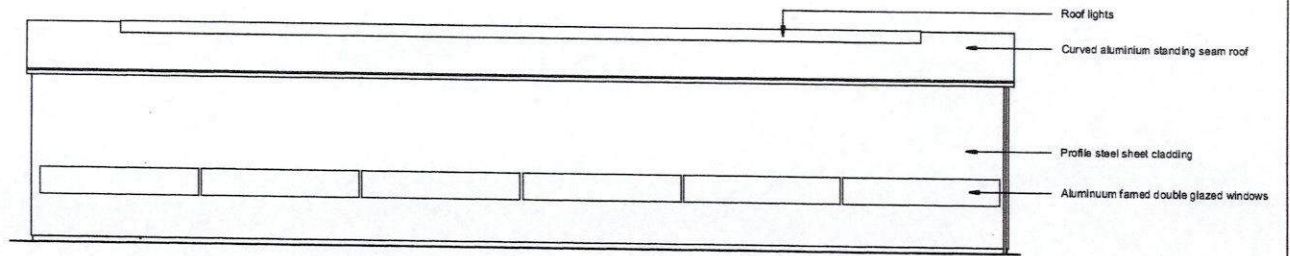
Elevation C
