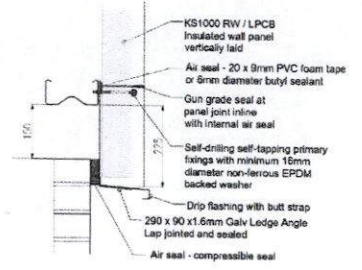
DRIP DETAIL AT F.F.L
