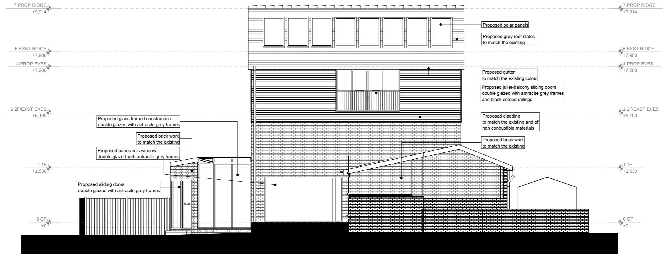
PROPOSED SIDE ELEVATION-SOUTH-(NO FENCE)
