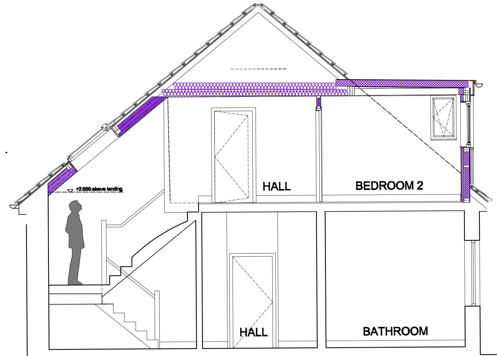
Proposed Section BB 1:50 @ A3
