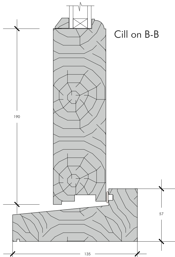
Proposed Door Section Detail
