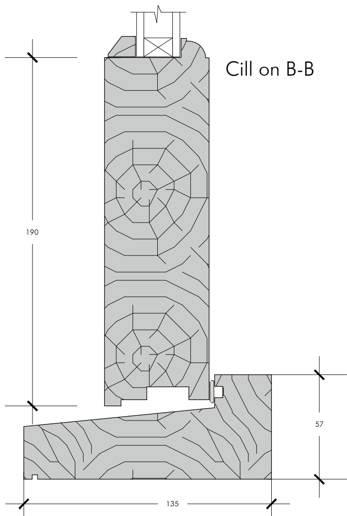
Existing Door Section Detail
