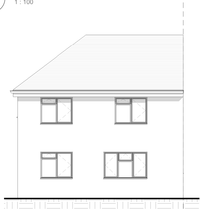
3 Existing Rear Elevation 1 : 100
