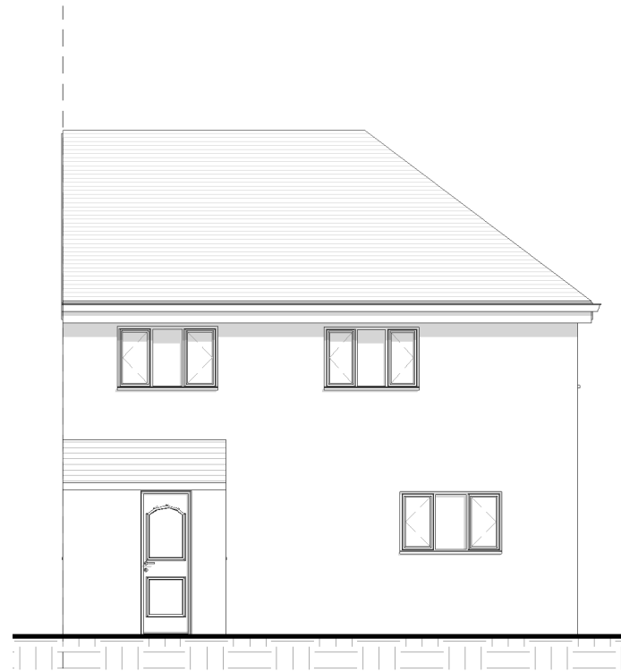
1 Existing Front Elevation 1 : 100
