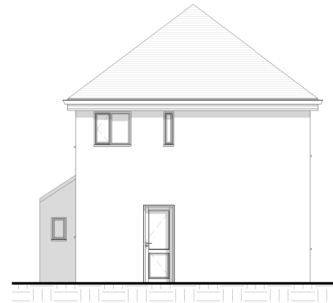
2 Existing Side Elevation-Right 1 : 100
