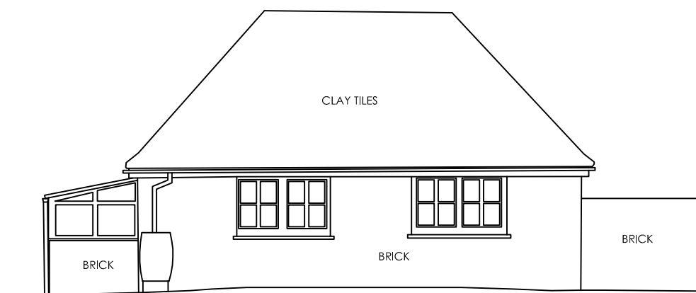
GARAGE - SOUTH ELEVATION
