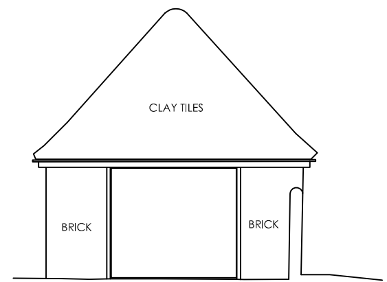
GARAGE - EAST ELEVATION
