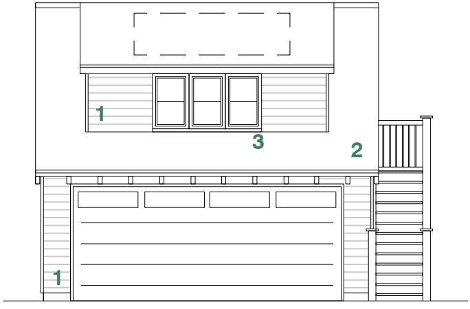
GARAGE PROPOSED SOUTH ELEVATION SCALE 1:100 @ a3
