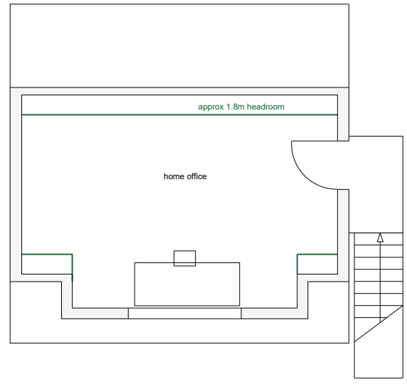
GARAGE PROPOSED ROOF SPACE PLAN SCALE 1:100 @ a3
