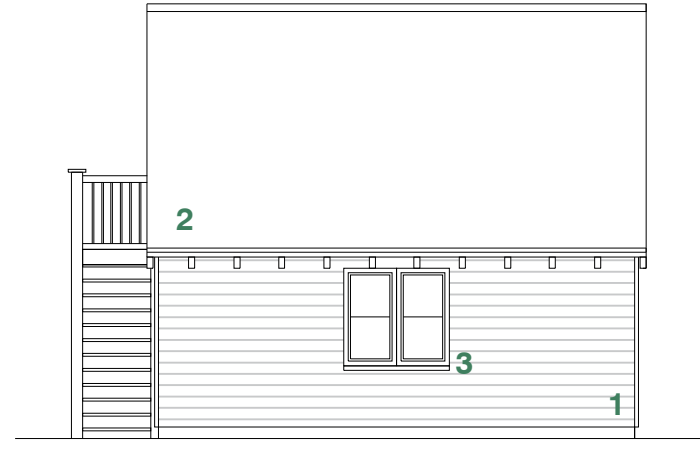
GARAGE PROPOSED NORTH ELEVATION SCALE 1:100 @ a3
