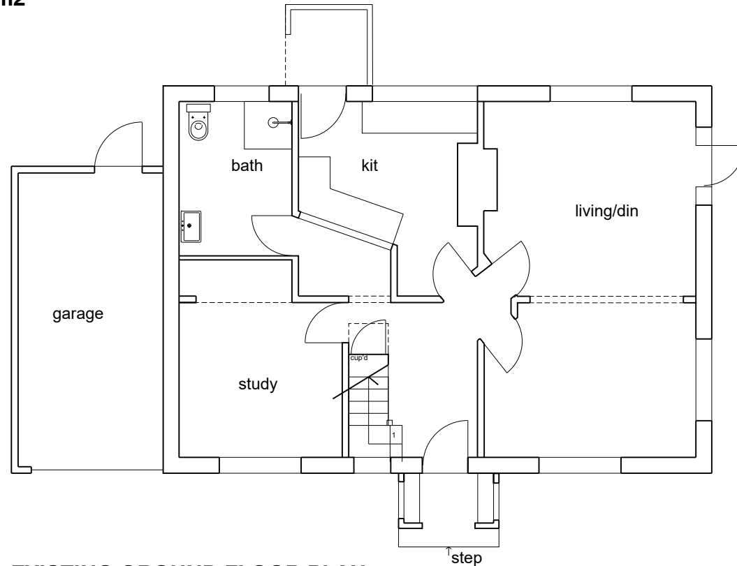
EXISTING GROUND FLOOR PLAN SCALE 1:100 @ a3
