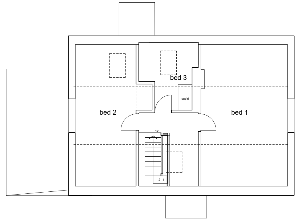
EXISTING FIRST FLOOR PLAN SCALE 1:100 @ a3
