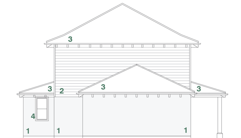
PROPOSED NORTH ELEVATION SCALE 1:100 @ a3
