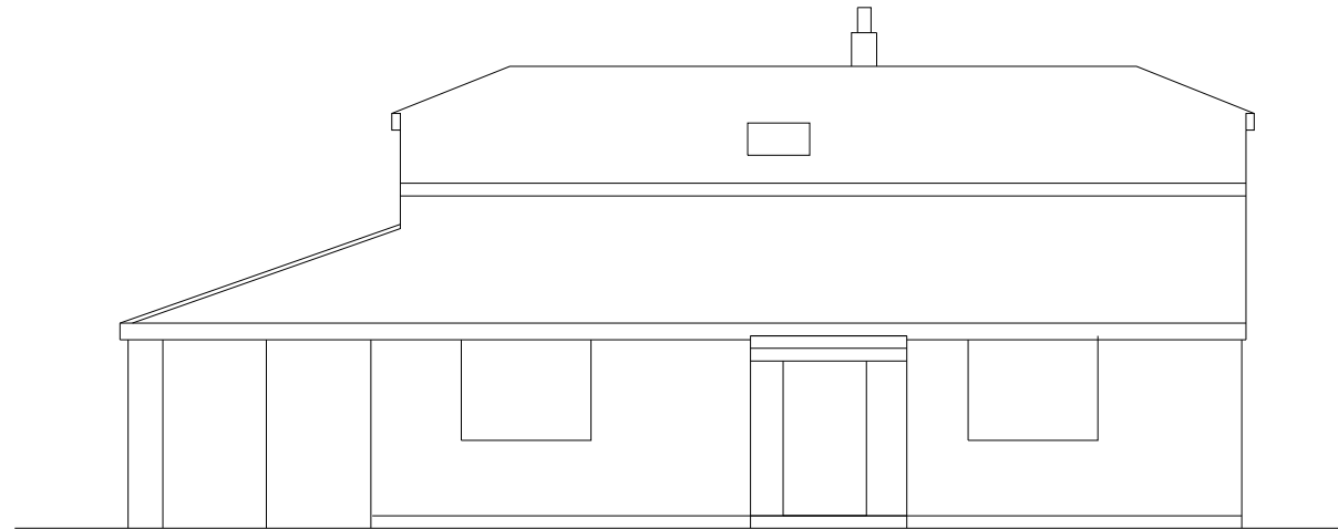
EXISTING NORTH ELEVATION SCALE 1:100 @ a3
