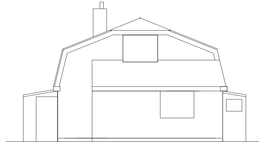
EXISTING EAST ELEVATION SCALE 1:100 @ a3
