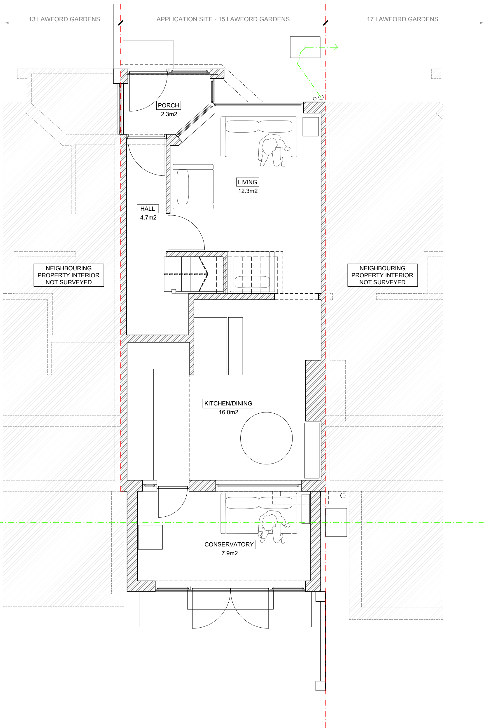
EX 01 Existing Ground Floor Plan
