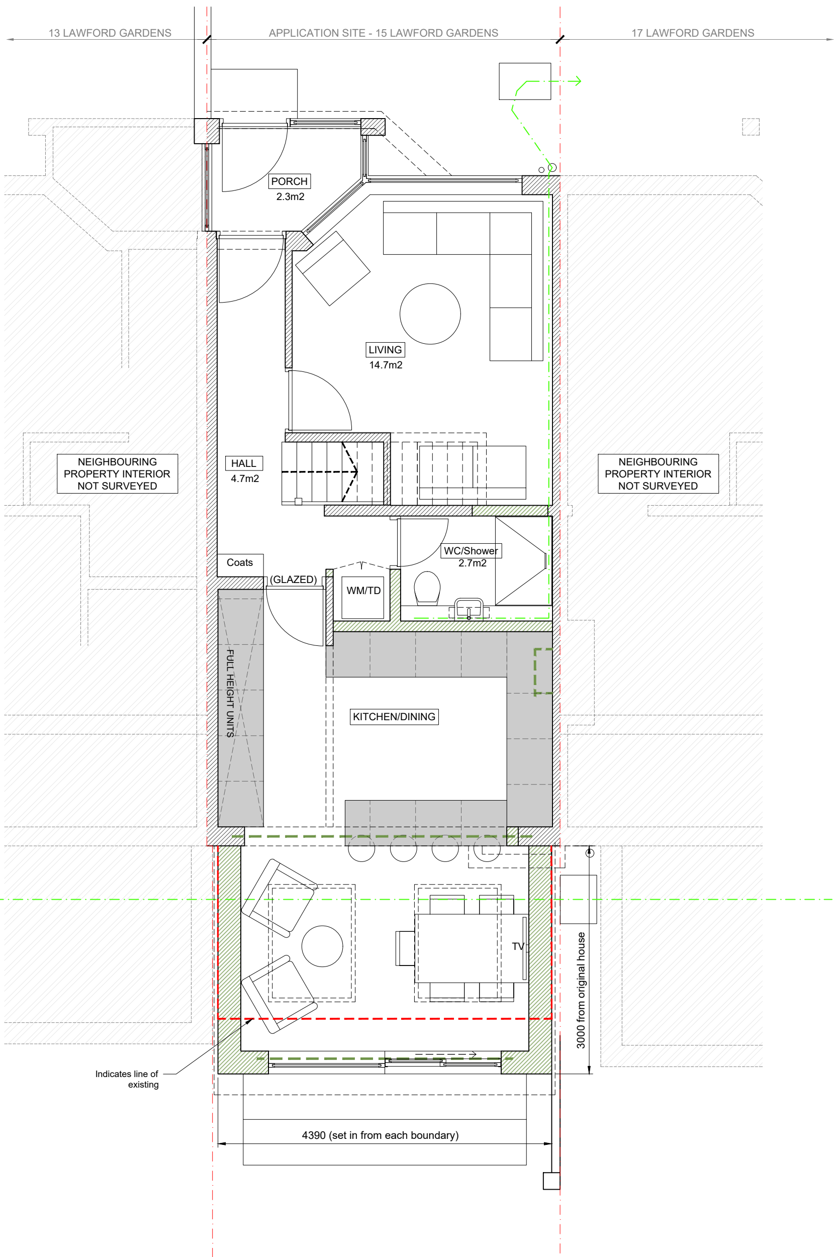
GA 01 Proposed Ground Floor Plan
