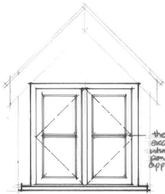
DORMER WINDOWS (FRONT) 1:20
