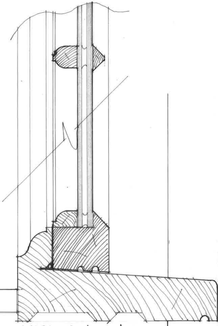
TYPICAL SECTION 1:2
