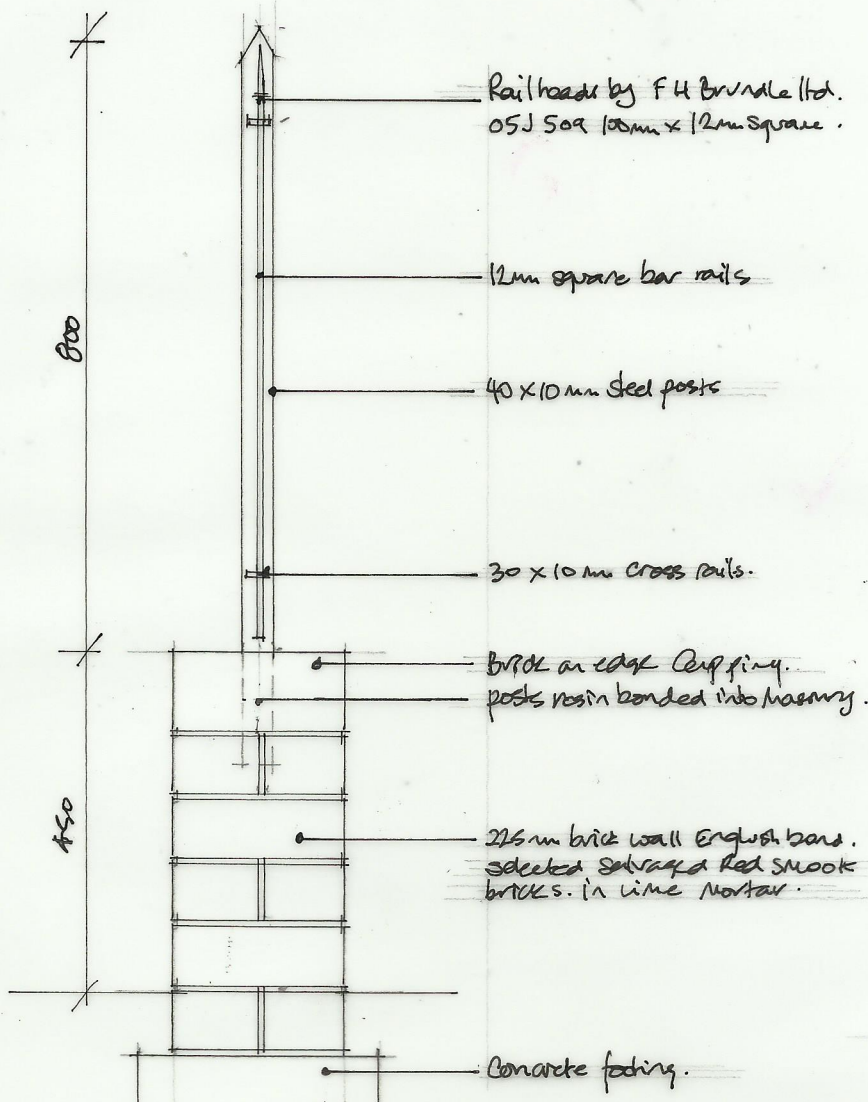
SECTION THRU NEW WALL 1:10
