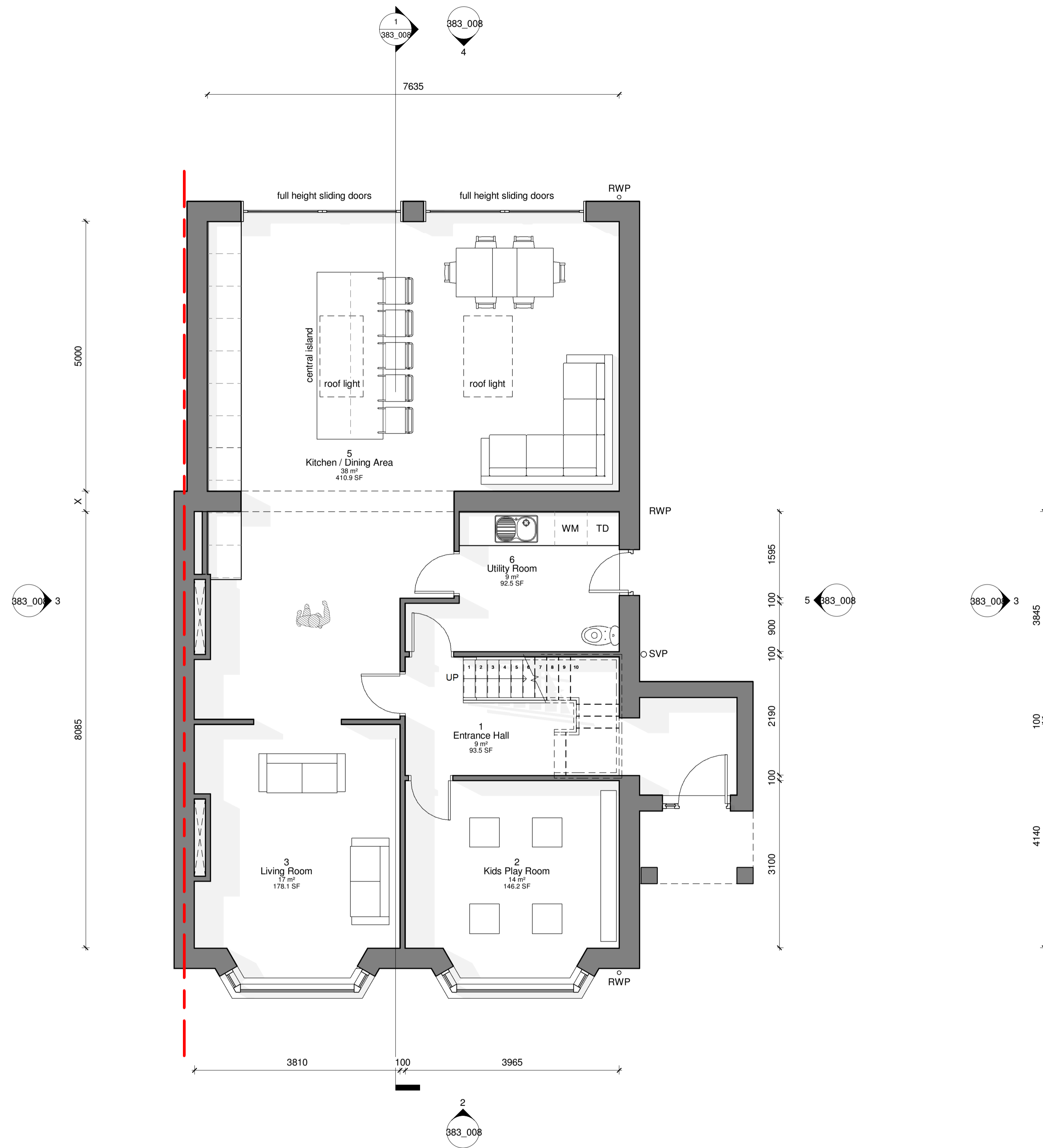
1 00 Ground Floor (PROPOSED) 1 : 50
