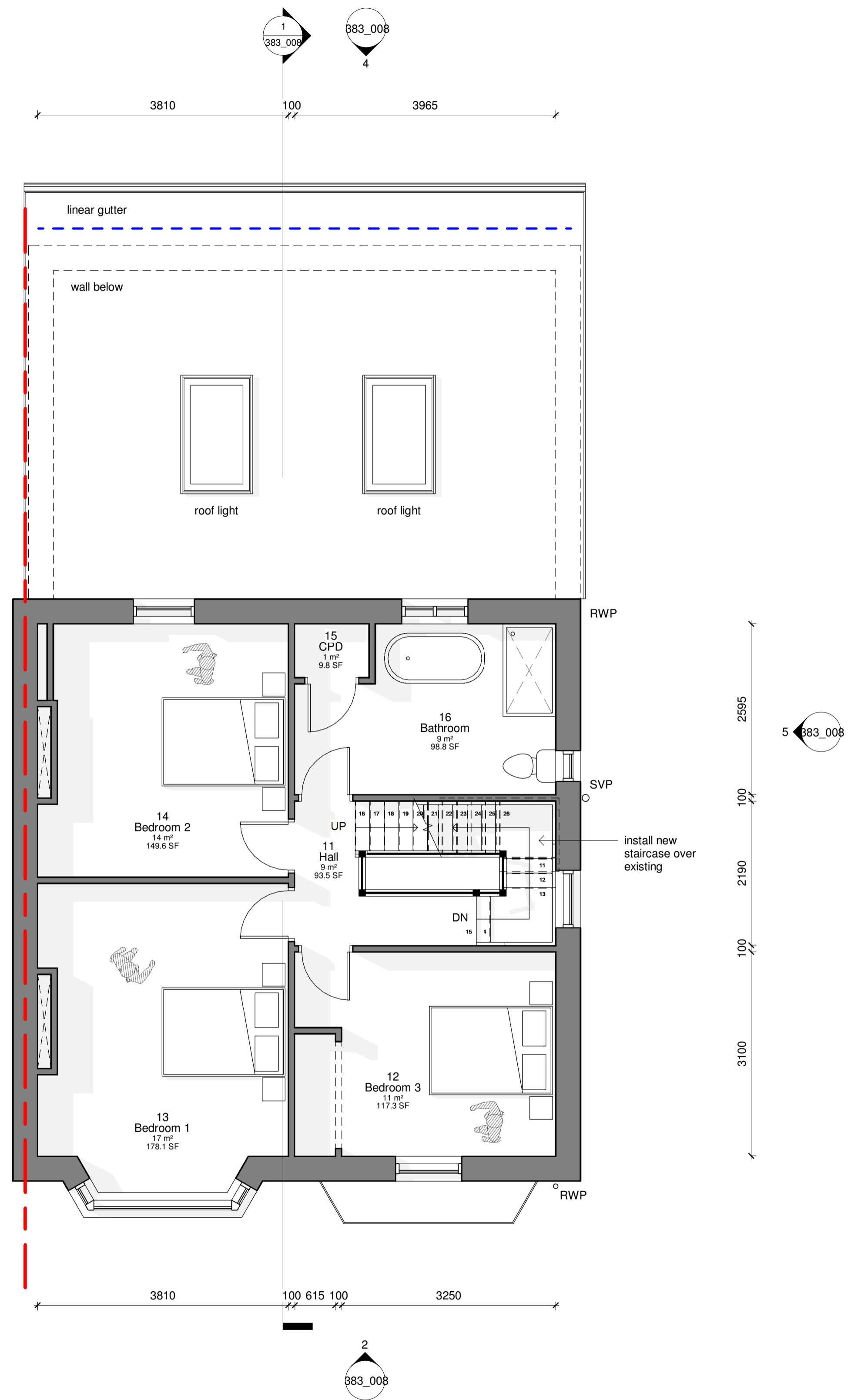
2 01 First Floor (PROPOSED) 1 : 50
