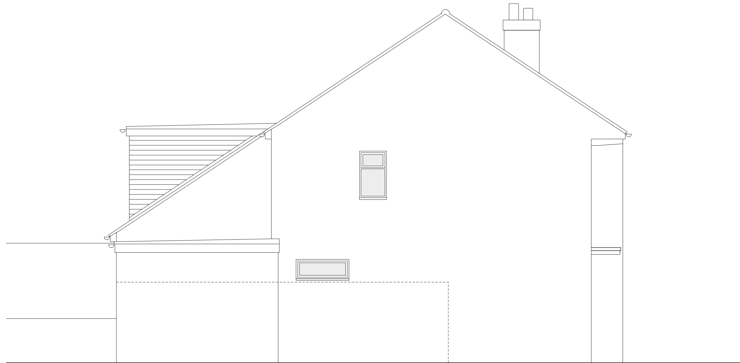
Existing Side Elevation scale 1:50 @ A2
