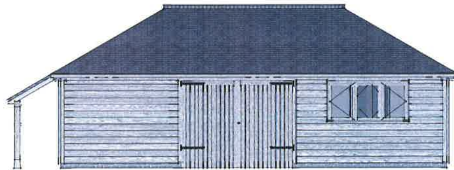
PROPOSED SOUTH-WEST ELEVATION
