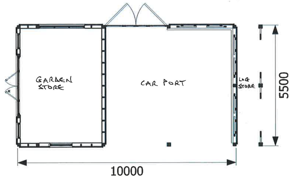
PROPOSED FLOOR PLAN
