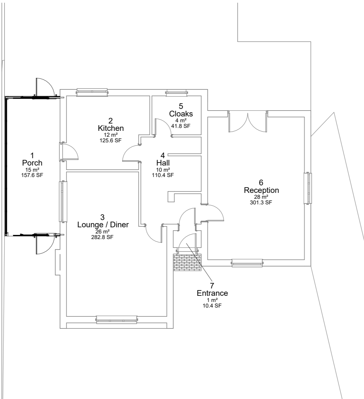
1 Level 0 Proposed 1 : 100
