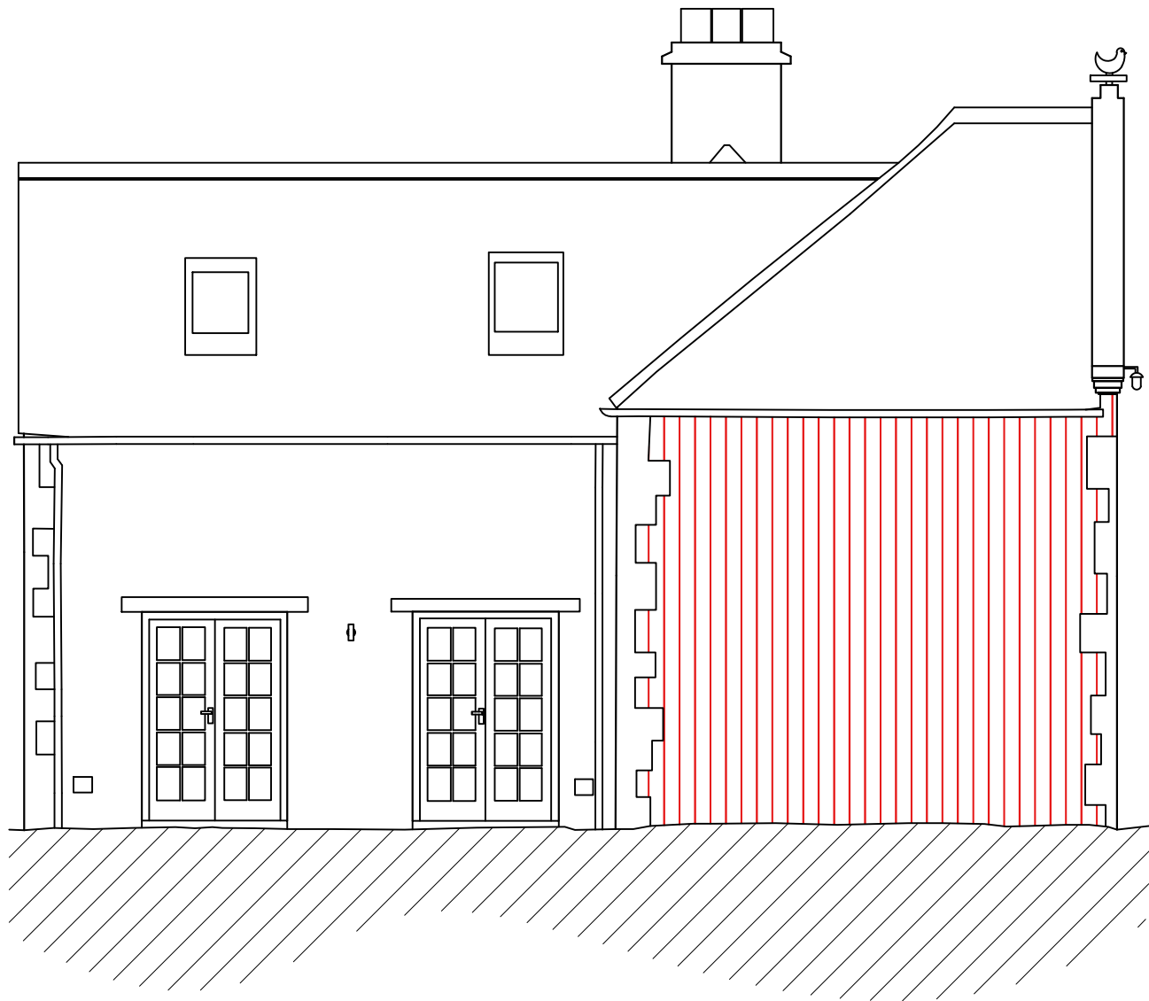
SOUTHWEST ELEVATION
