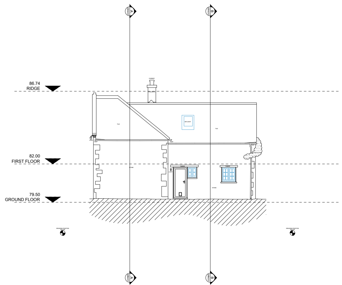
NORTHEAST ELEVATION
