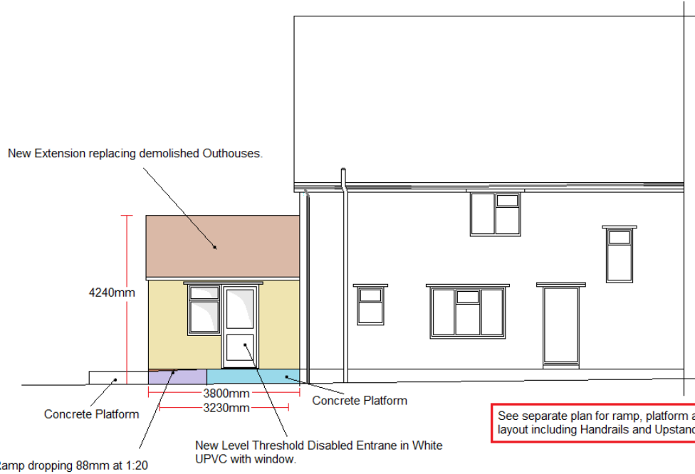
Proposed Front Elevations 1-100
