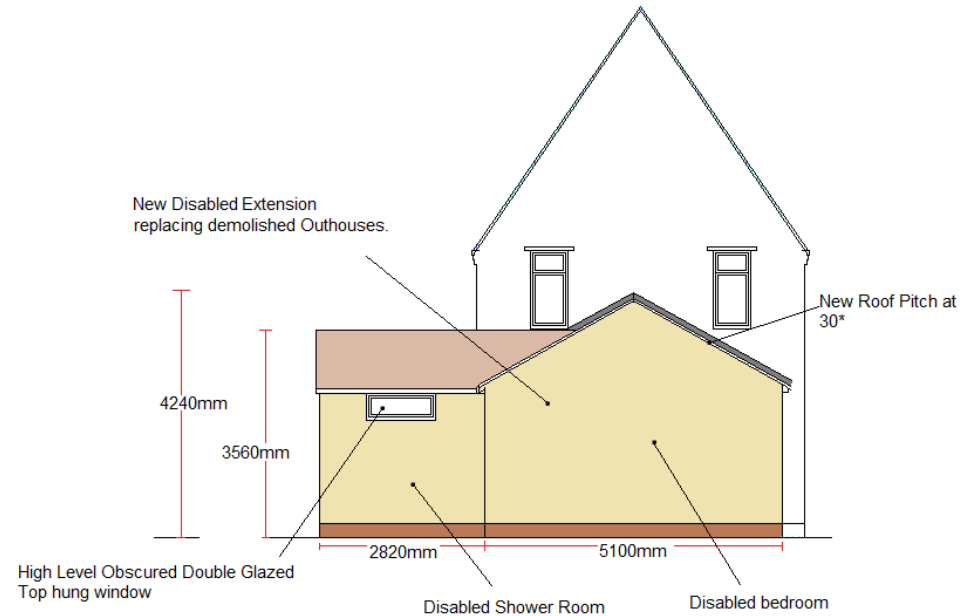
Proposed Side 1 Elevation 1-100
