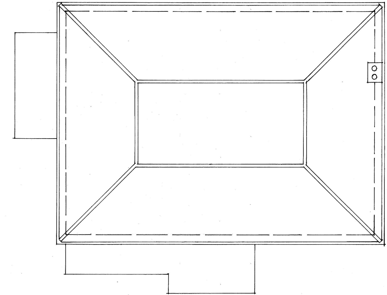
ROOF PLAN
