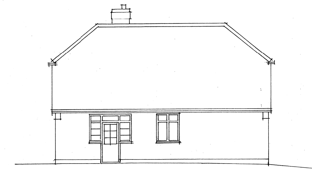
SIDE SOUTH EAST ELEVATION
