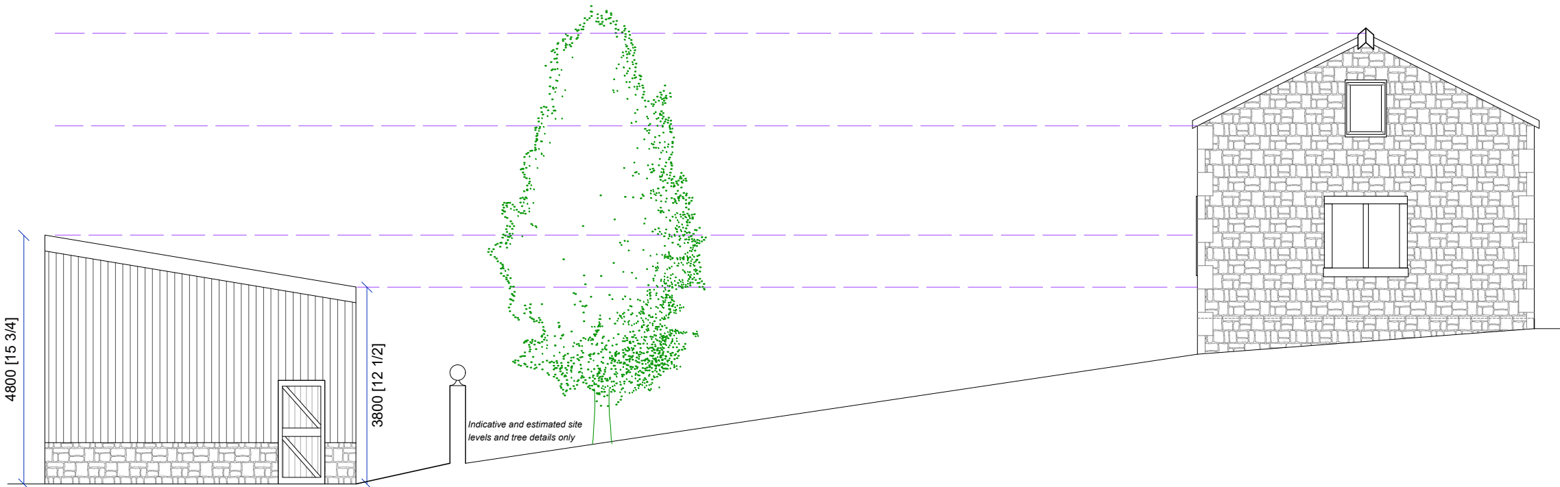
Proposed Site Section Comparison to existing building on site
