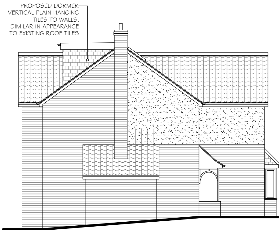
SIDE ELEVATION
